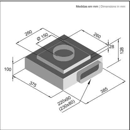
MOT 855 F INTERIOR | INDOOR
